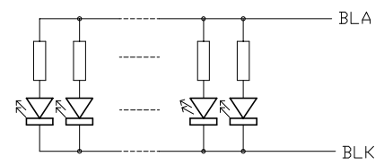
Backlight Circuit (No. of LEDs = 12pcs) Scale=free
